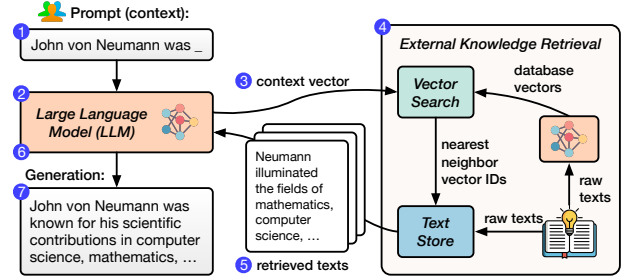
Figure 1: A retrieval-augmented language model (RALM).
